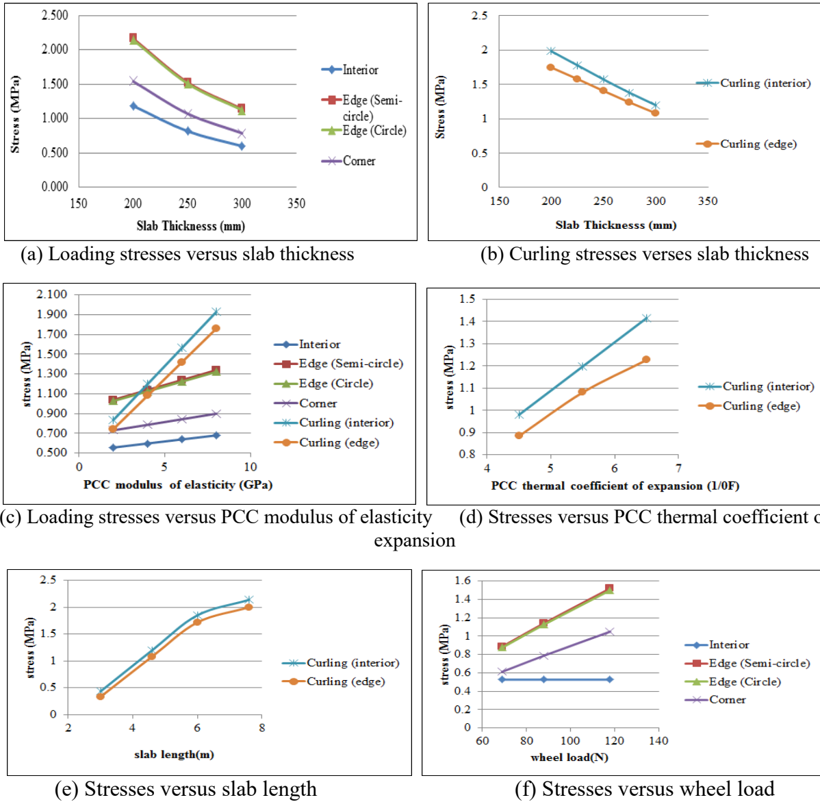
Fig. 3. Results of sensitivity analysis for stresses at different locations.
