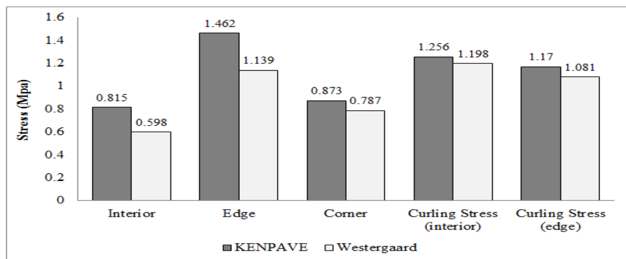
Fig. 2. Comparison of stresses between Westergaard and KENPAVE method.
