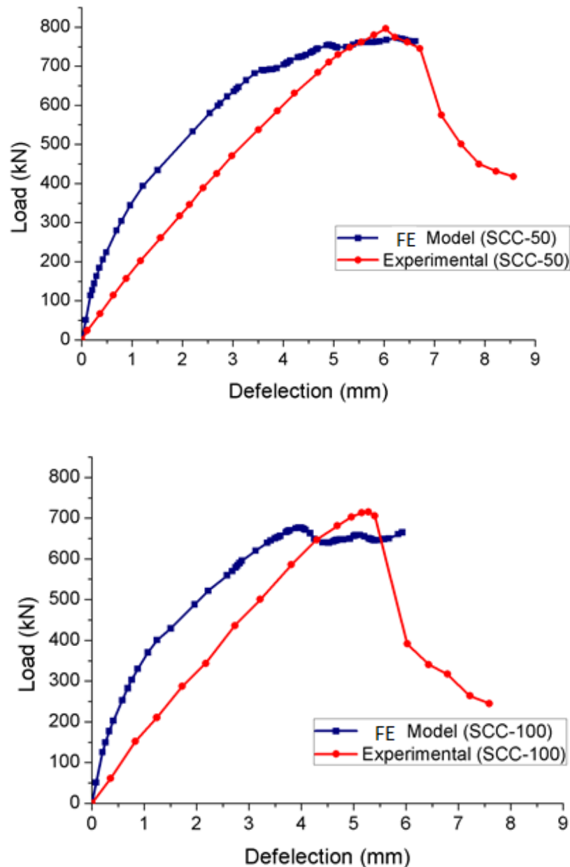
Fig. 10. FE model versus experimental load-deflection curve for the beams.
