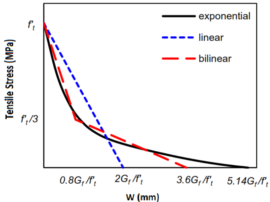
Fig. 5. Stress-crack width for concrete in tension [18].
