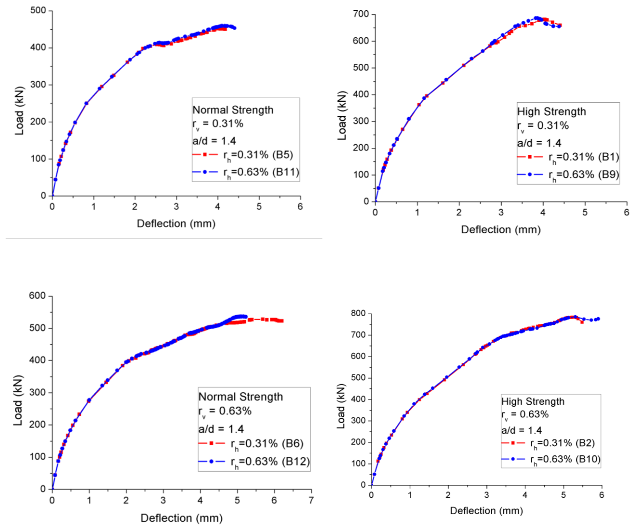
Fig. 14. Effect of r_h on the load-deflection response.
