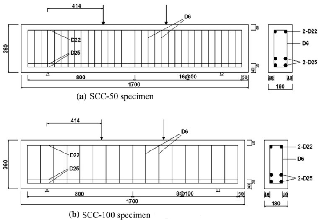
Fig. 2. Details and Dimensions of deep of beams (All dimensions in mm) [8].
