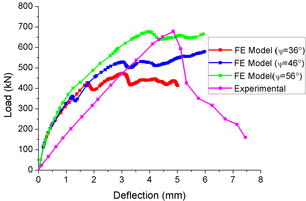
Fig. 8. Dilation angle sensitivity test.
