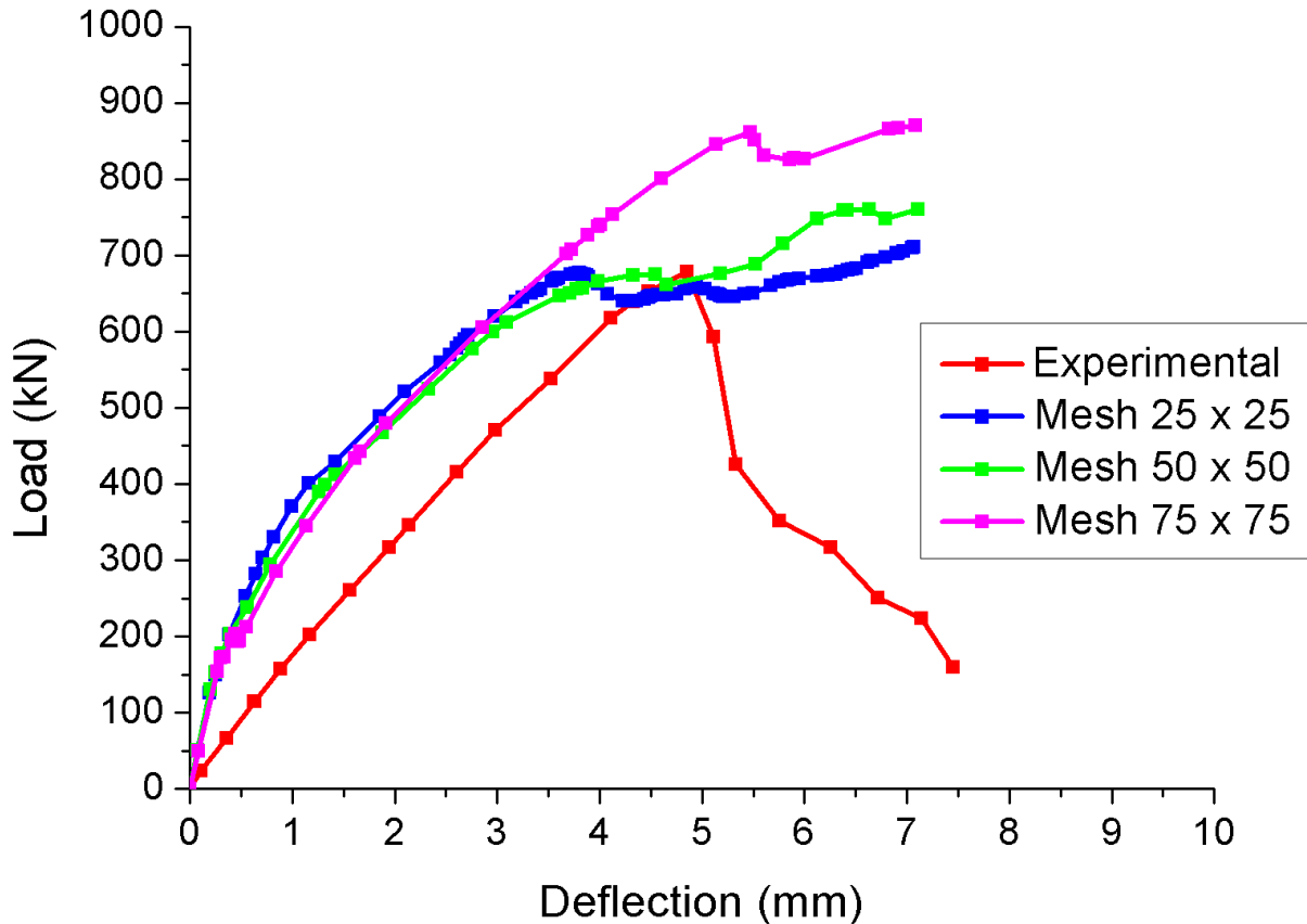
Fig. 9. Mesh sensitivity test.
