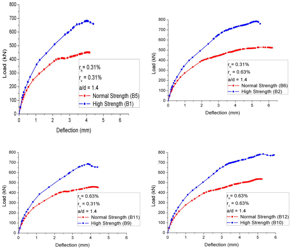
Fig. 12. Effect of f_c on the load-deflection response.
