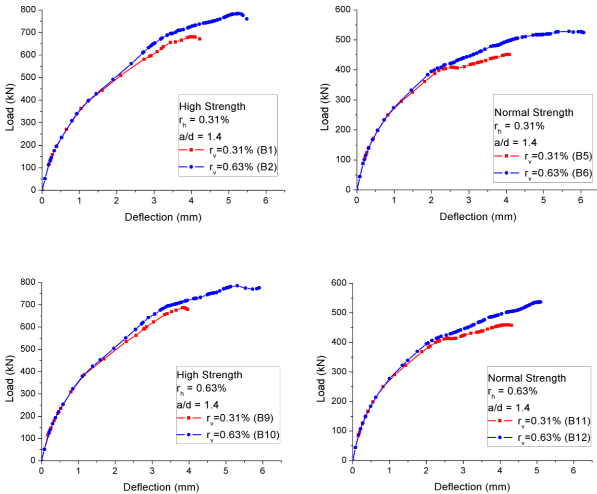
Fig. 13. Effect of r_v on the load-deflection response.
