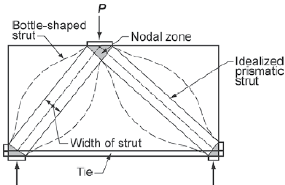
Fig. 1. Strut and tie model of deep beam [1]
