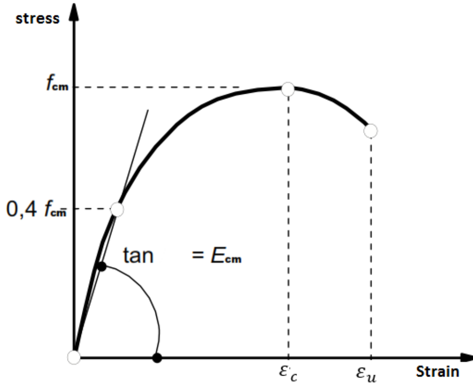
Fig. 4. Stress-strain model for concrete in compression [2].
