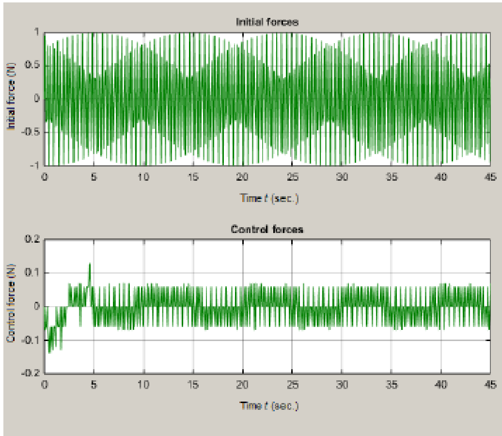
Fig. 10. The external and control forces with respect to time.
