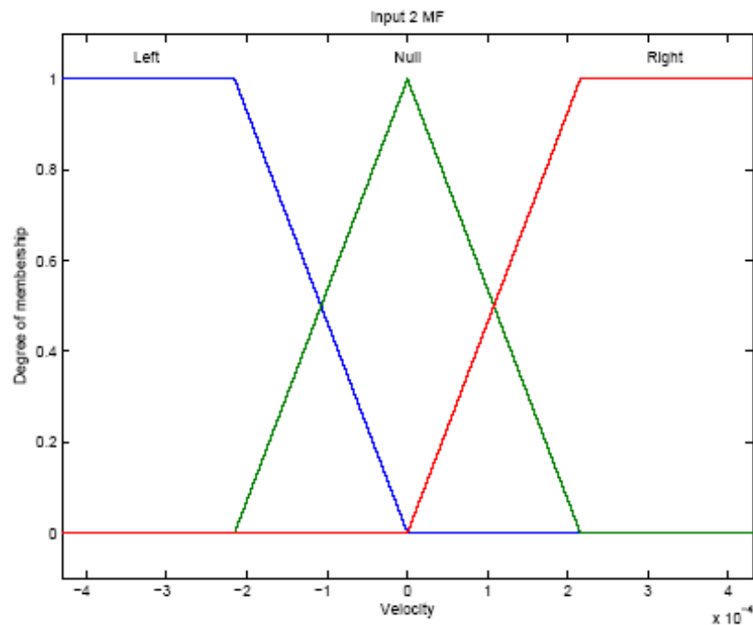
Fig. 2. Membership functions for the input (velocity) of the fuzzy inference system.
