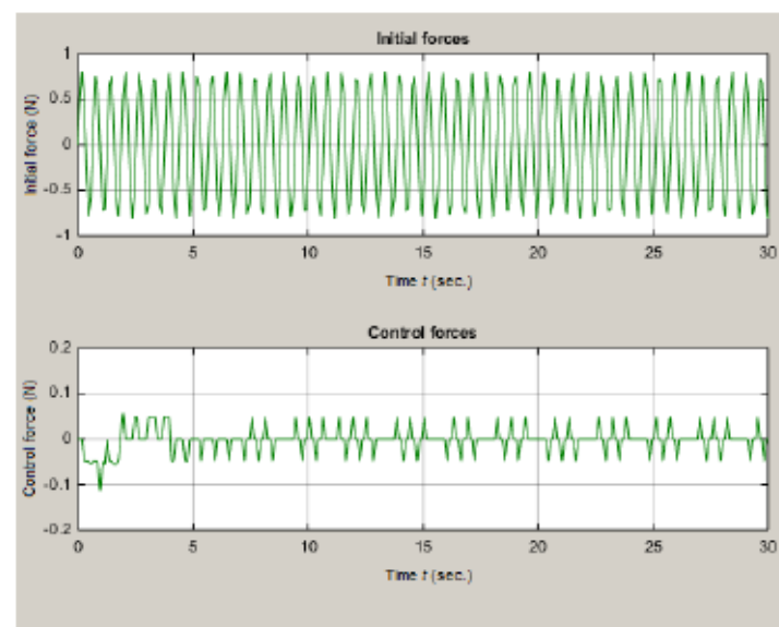
Fig. 7. The external and control forces with respect to time.
