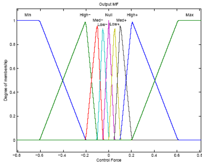
Fig. 3. Membership functions for the output (control forces) of the fuzzy inference system.
