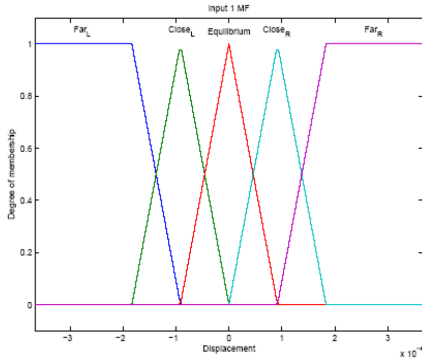
Fig. 1. Membership functions for the input (displacement) of the fuzzy inference system.
