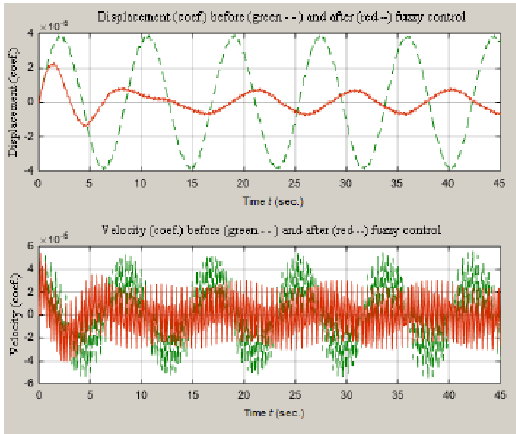
Fig. 9. Plots of the coefficients w^{11}(t) , w_t^{11}(t) (characteristics of displacement and velocity) before and after the control
