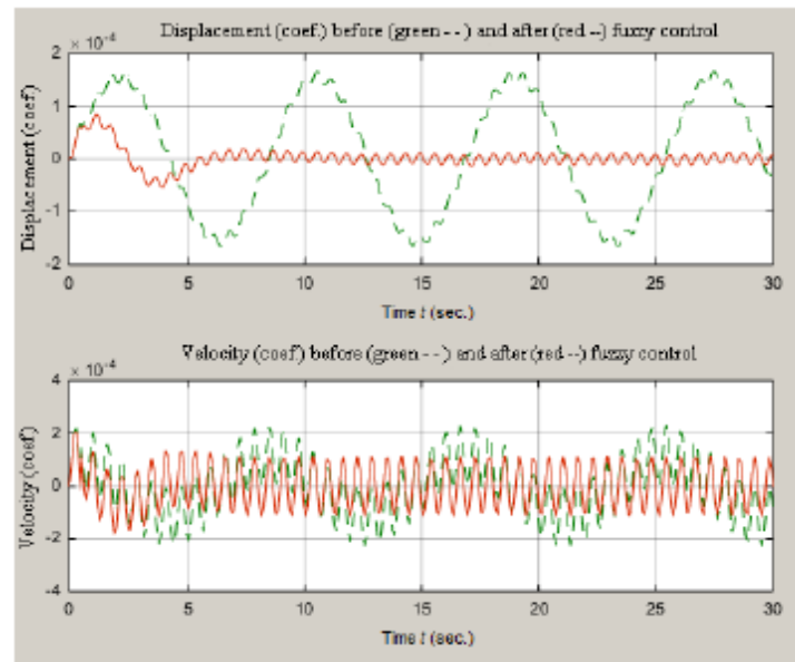
Fig. 6. Plots of the coefficients w^{11}(t) , w_t^{11}(t) (characteristics of displacement and velocity) before and after the control.
