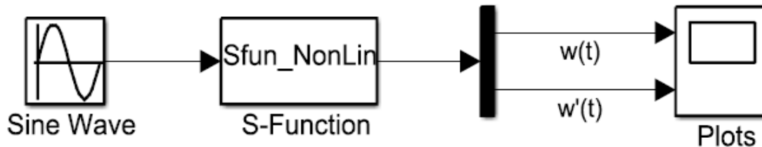
Fig. 4. The initial model-diagram for the nonlinear system
