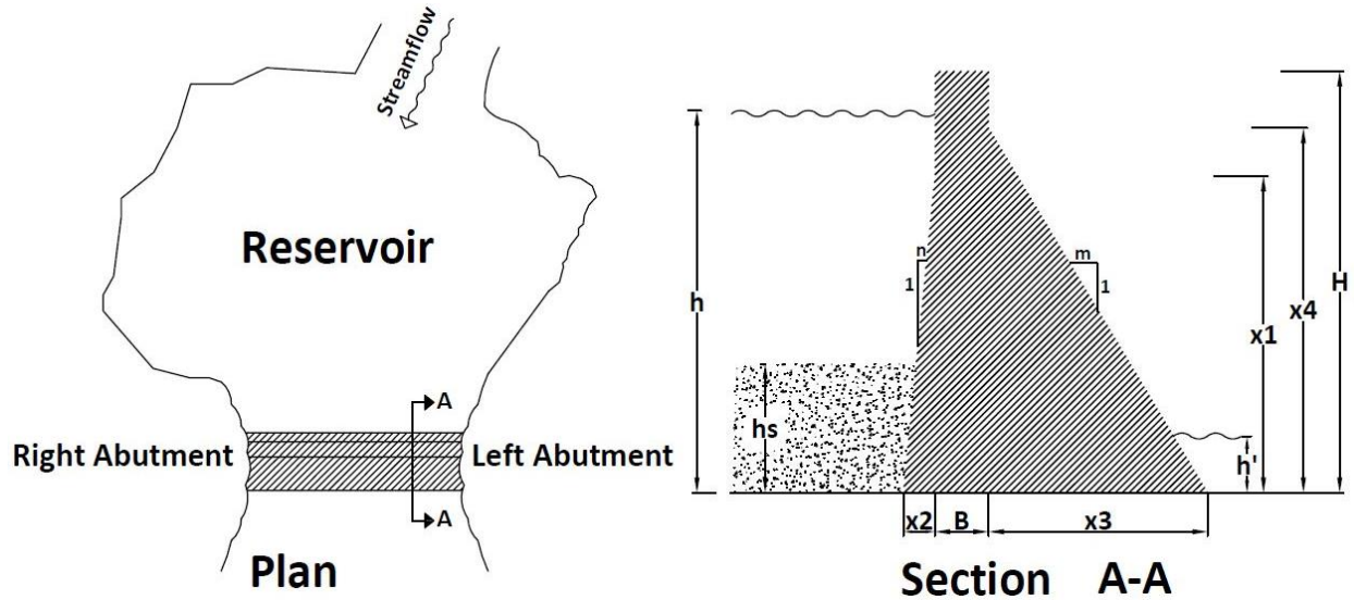
Fig. 1. A gravity dam schematic including geometric parameters.
