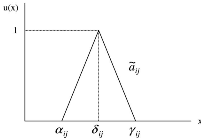
Fig 1. Triangle Membership function in Fuzzy – Delphi Method [19].
