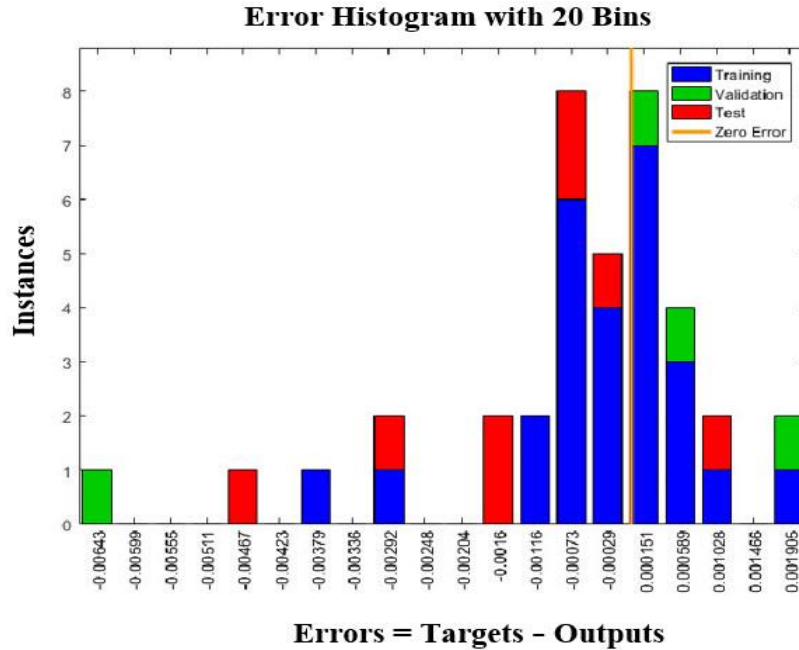
Fig. (4). Histograms of errors for all data set using MLP model
