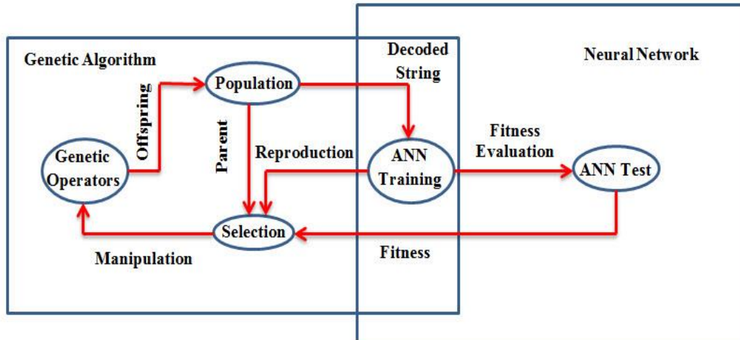
Fig. (5). The structure of hybrid GA-ANN flowchart [40]
