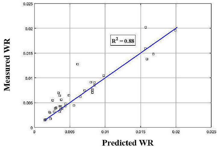
Fig. (2). R^2 of predicted and measured WR values for all data set using MLP model
